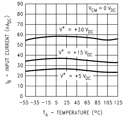
Input Current
