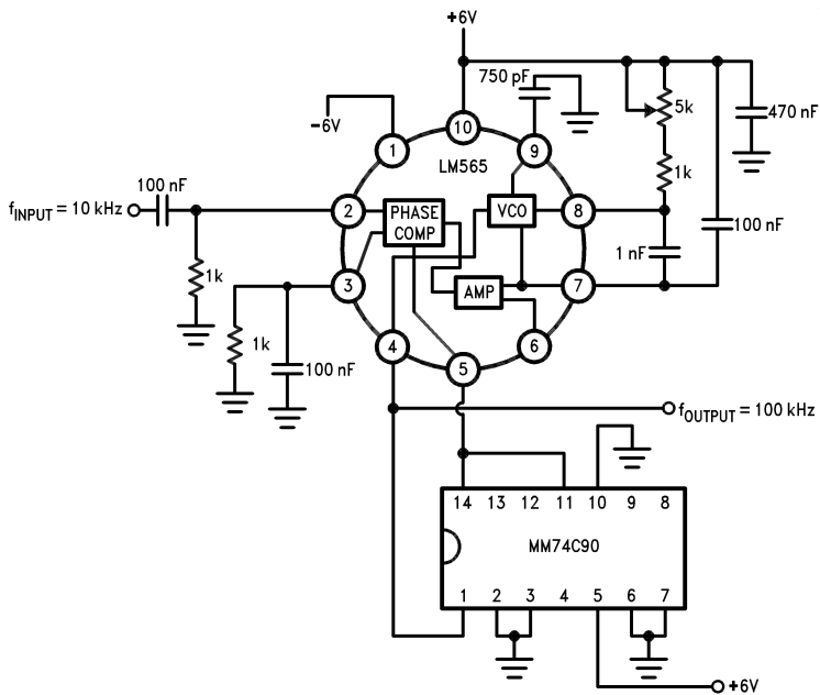
Figure 14. Frequency Multiplier (x10)
